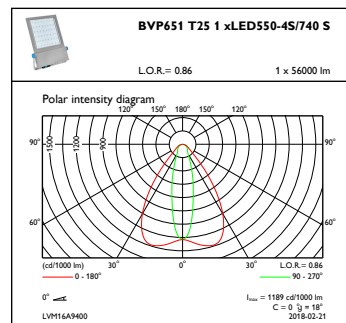
OFPC1_BVP651T251xLED550-4S740S
