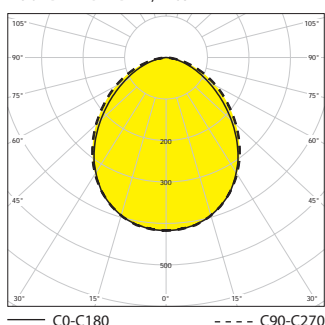
HOUND-MAG-LED-4K, IP 65
