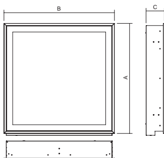
HOUND-MAG-LED-4K, IP 65
