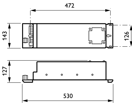
GearUnits ECB330/ECP330
