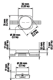
Clear Flat Lens
